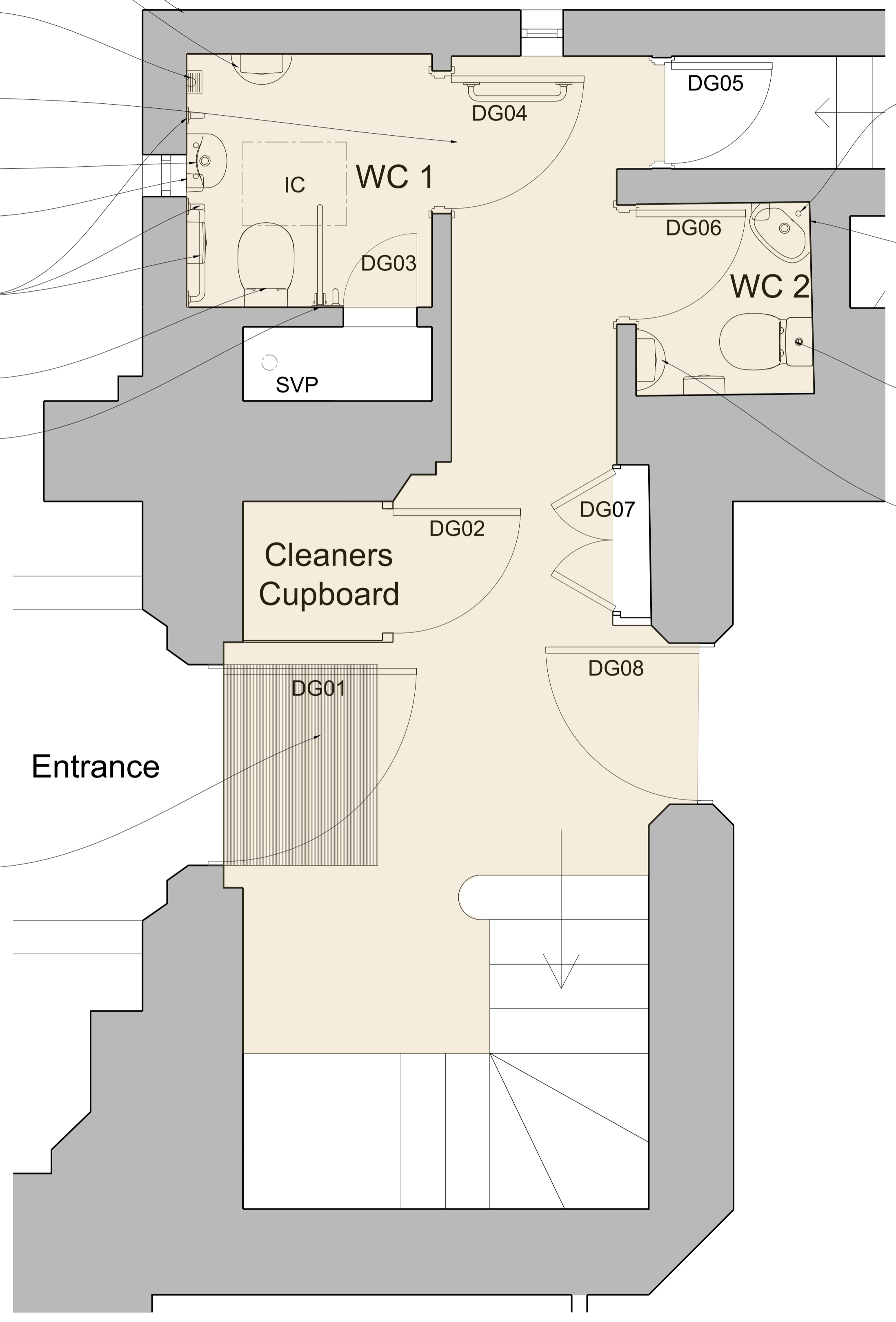
Ground Floor Part Plan 1:20 As Proposed
