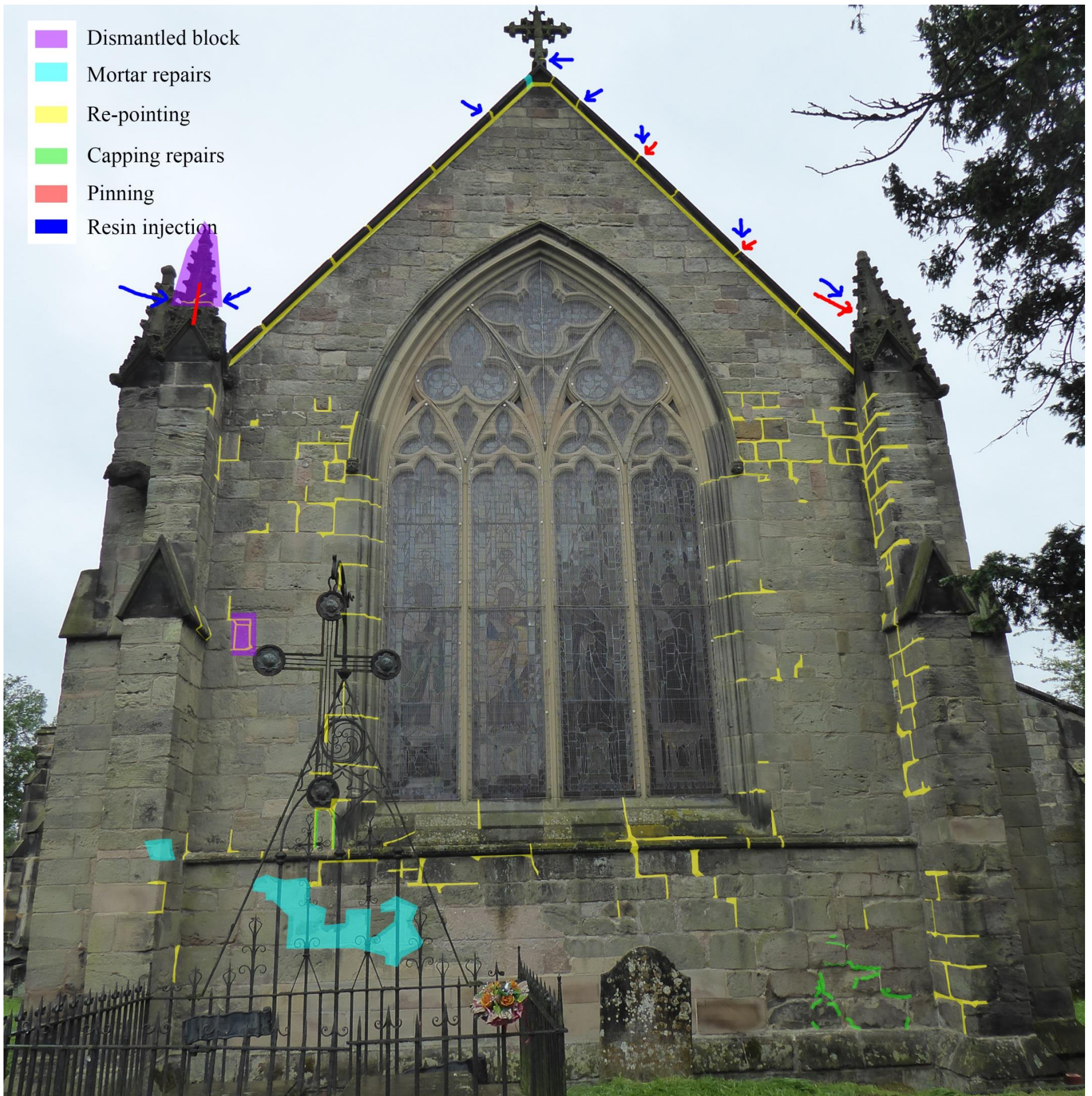
Conservation works mapping to Chancel exterior east wall
