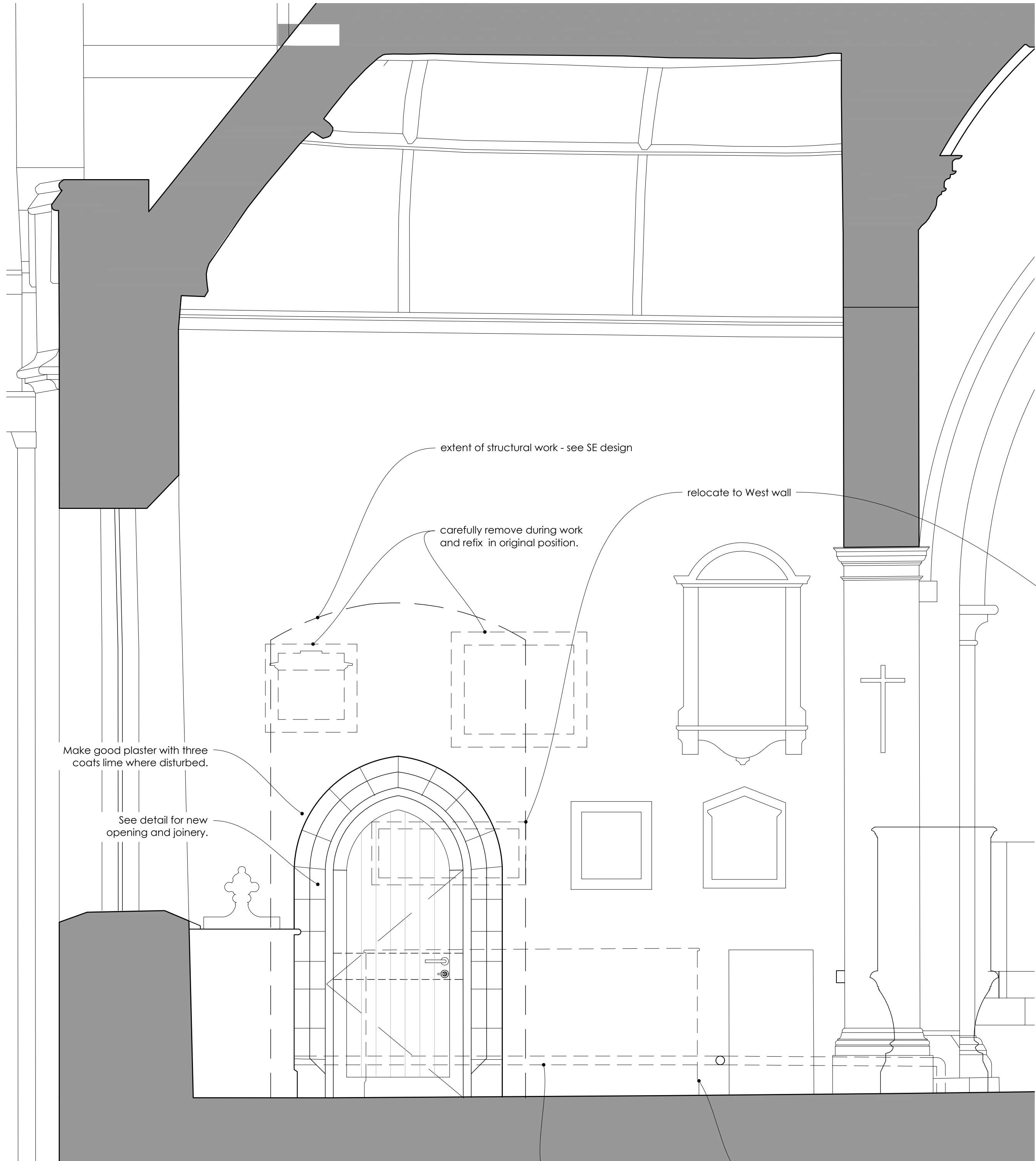
Proposed Elevation 1:20@A1
