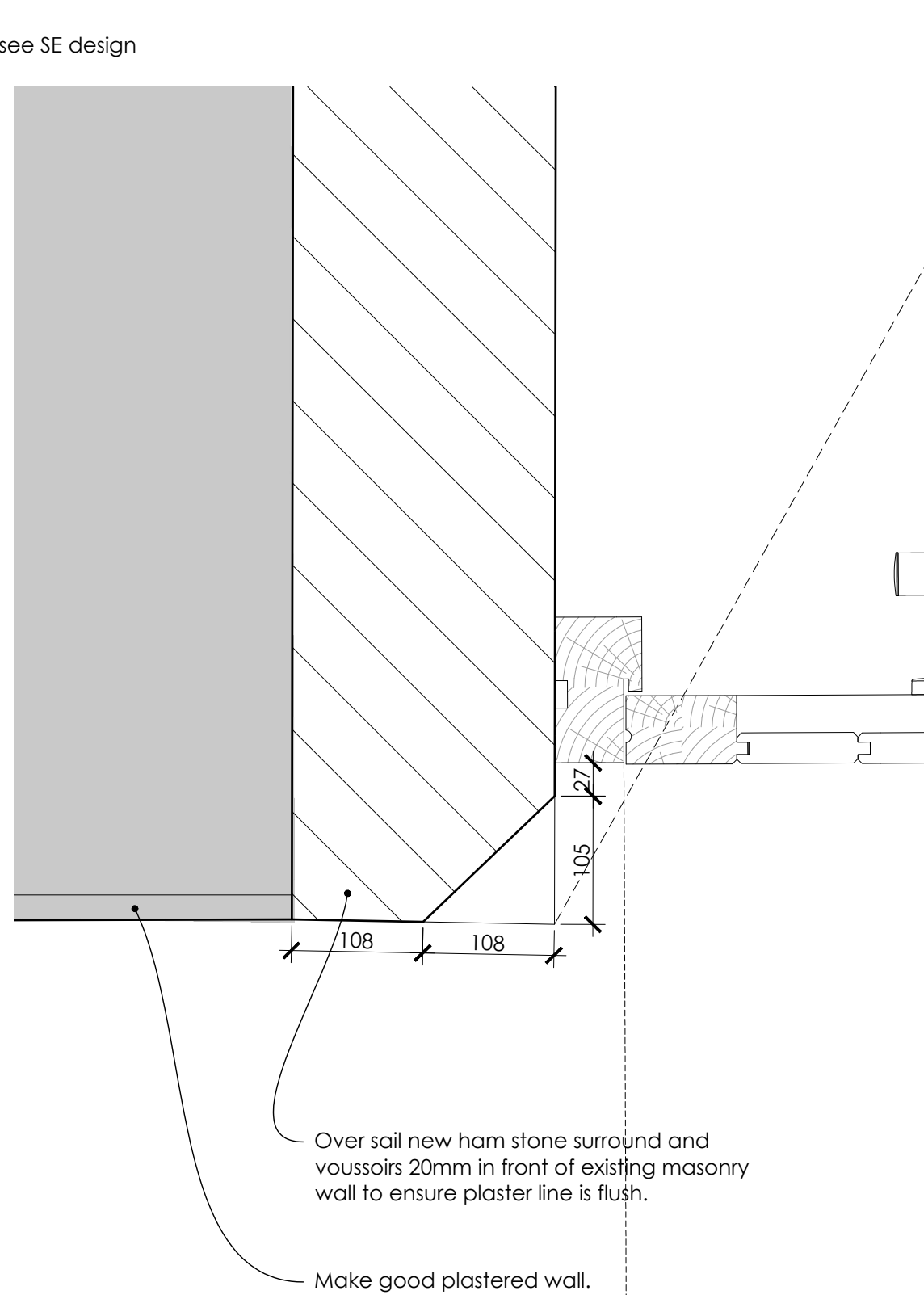
Ashlar surround detail 1:10@A1
