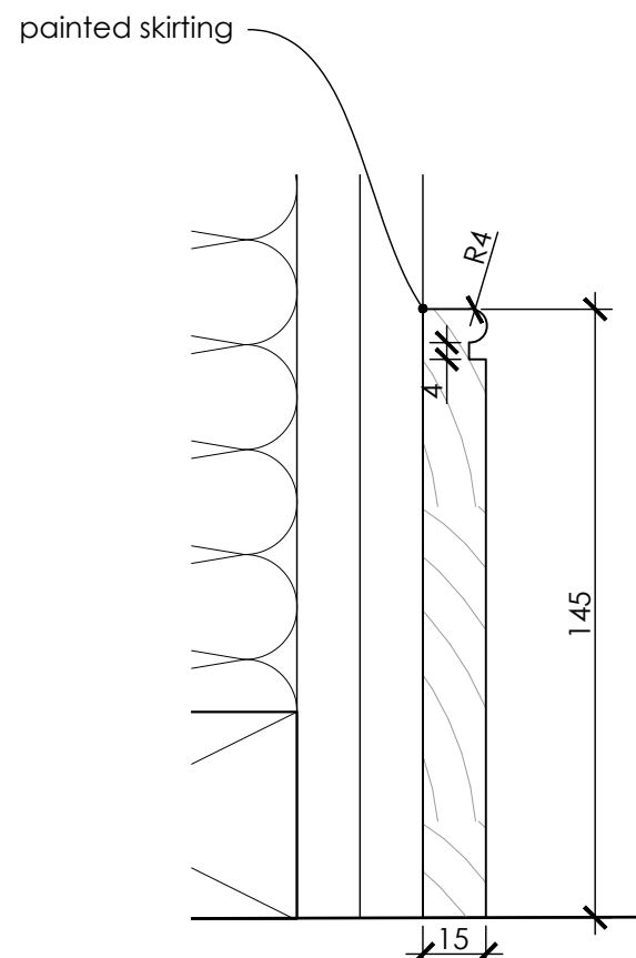
Skirting Detail 1:2@A1
