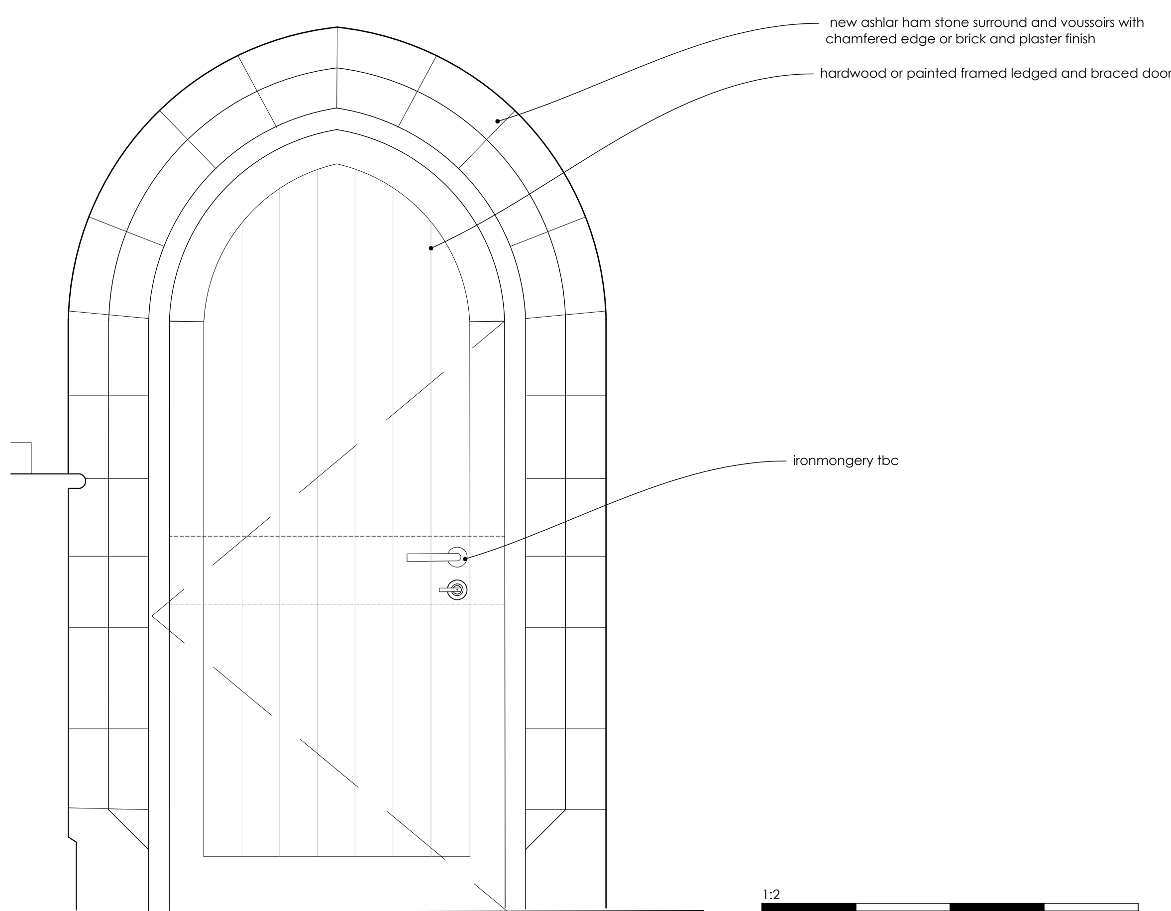
Elevation (Tansept side) 1:10@A1
