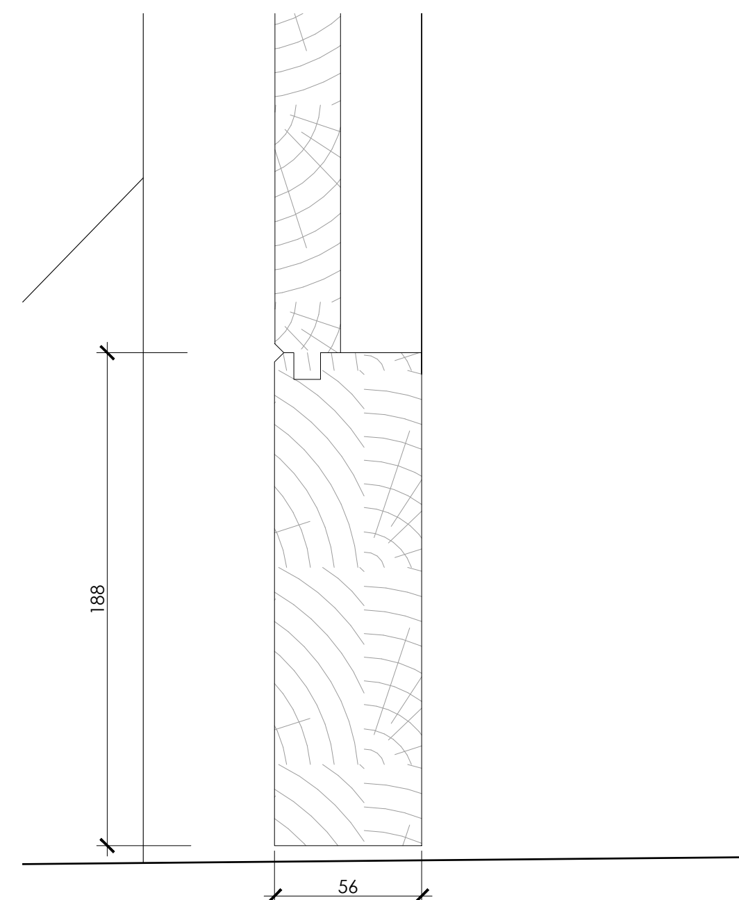
Section Detail 1:2@A1
