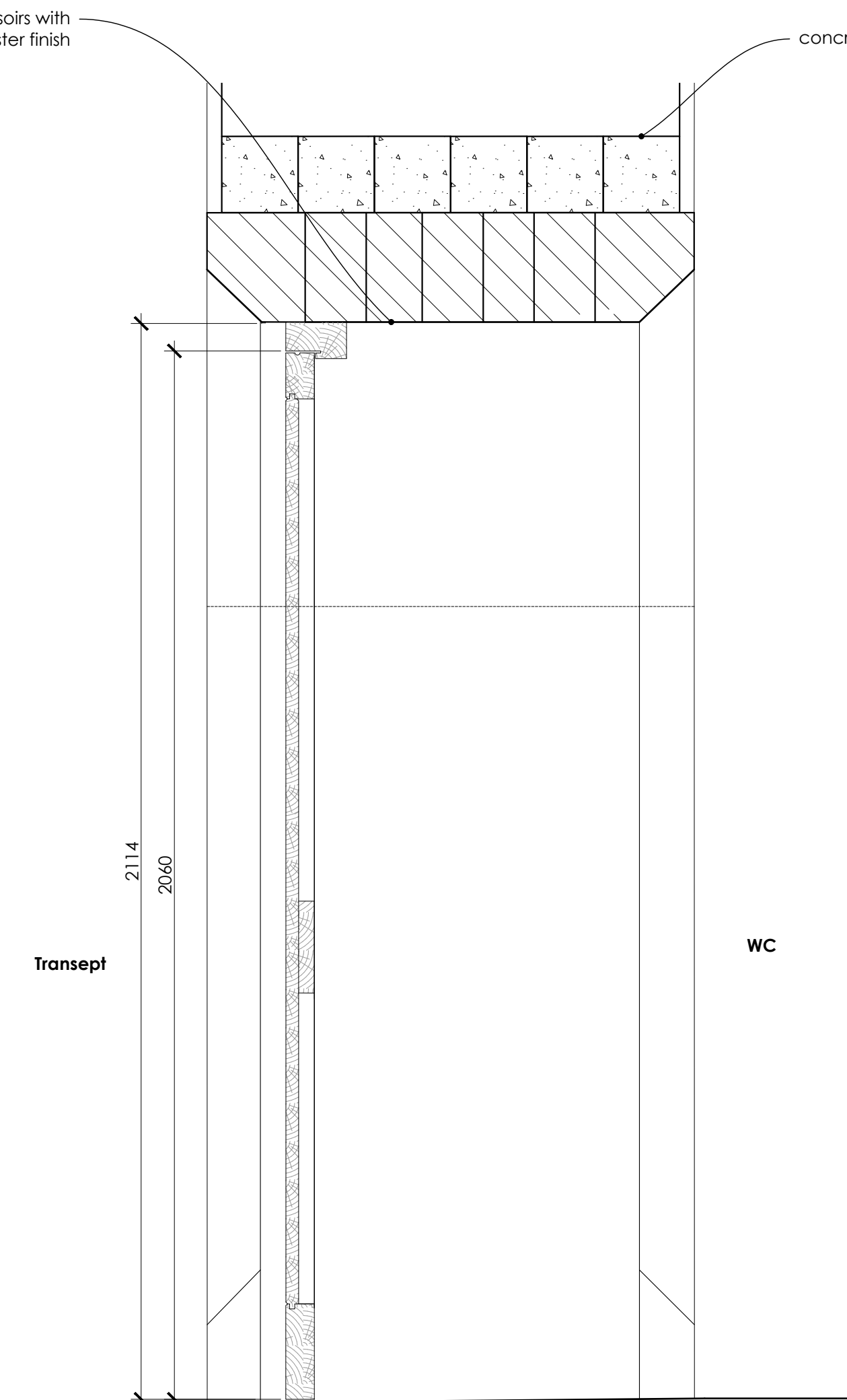
Section 1:10@A1
