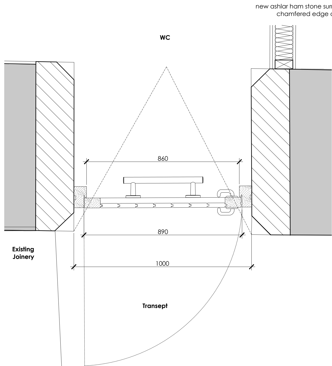
Plan 1:10@A1
