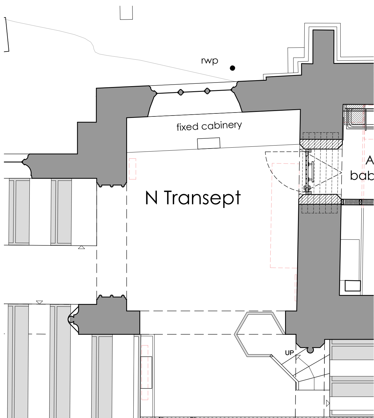
Proposed Plan 1:50@A1
