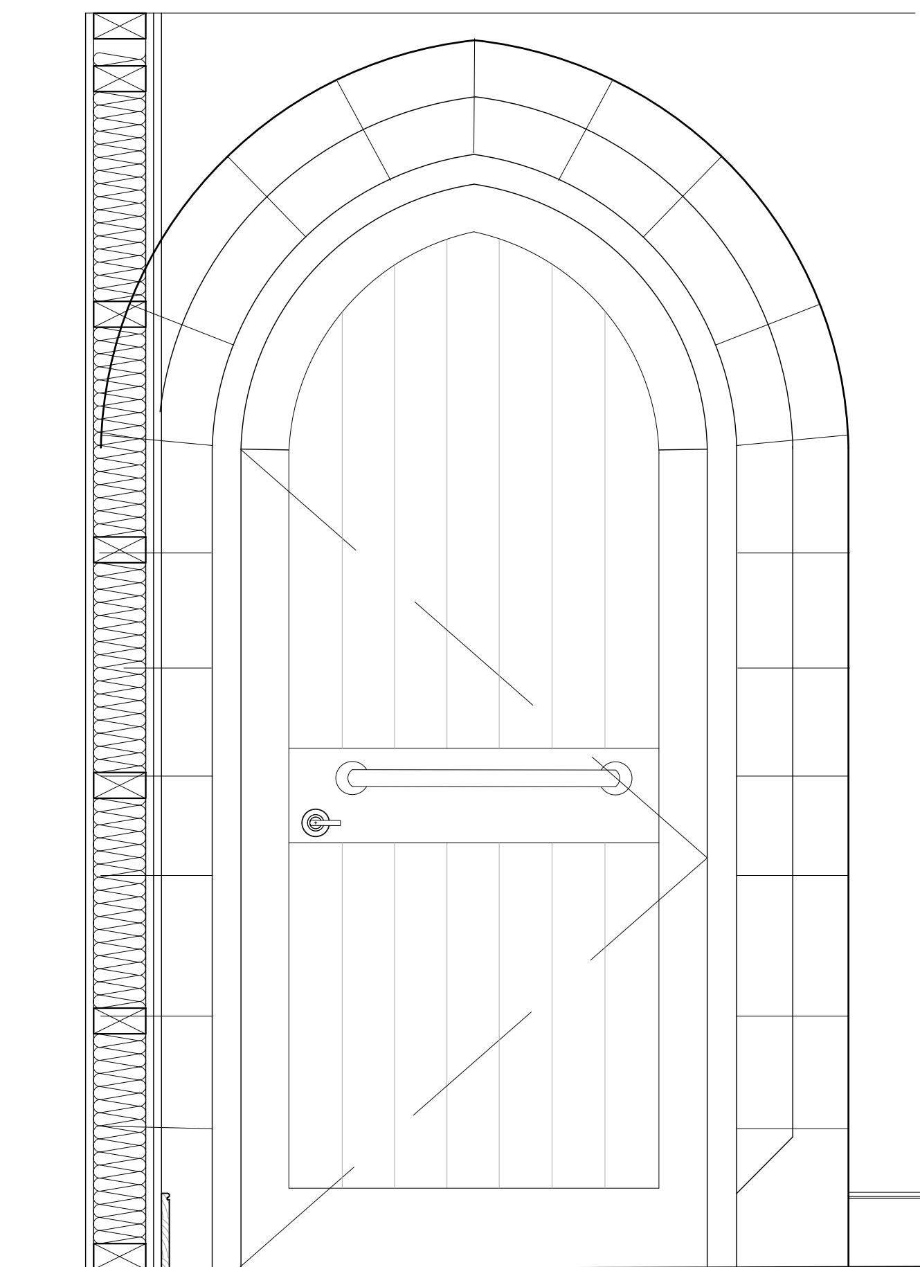
Elevation (WC side) 1:10@A1
