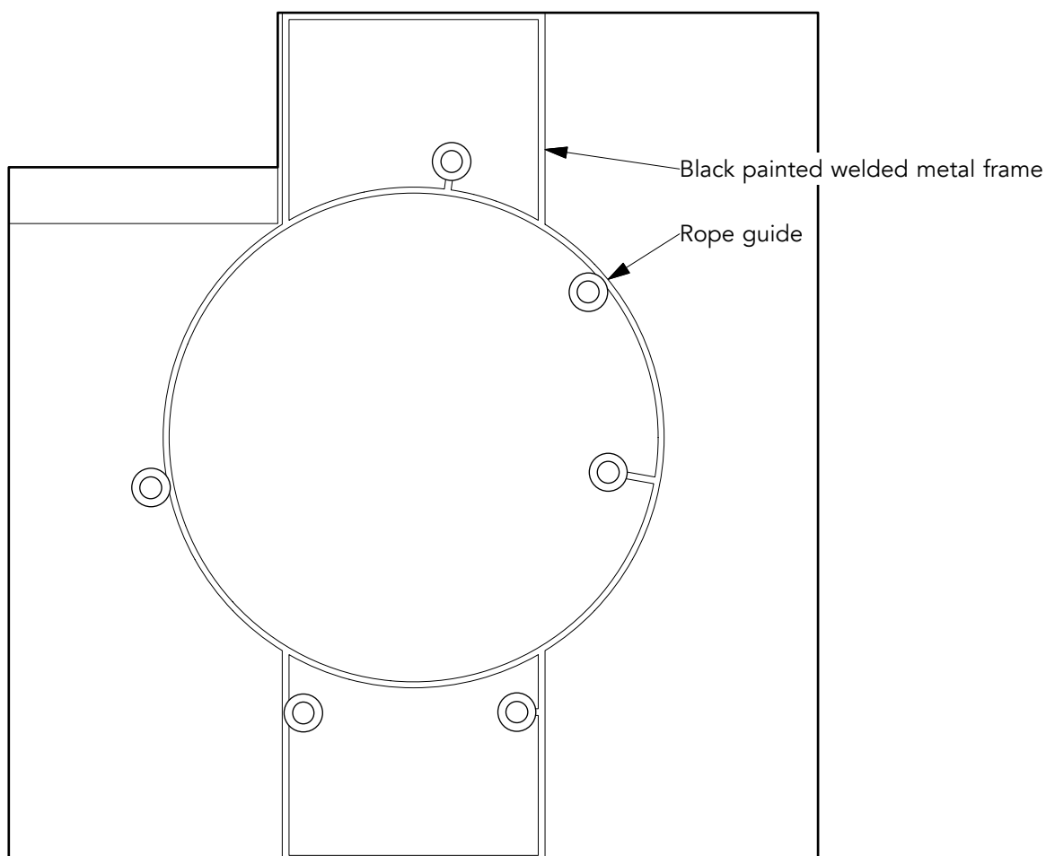
TEMPORARY BELL GUIDE FRAME POTENTIAL ARRANGEMENT 1:25
