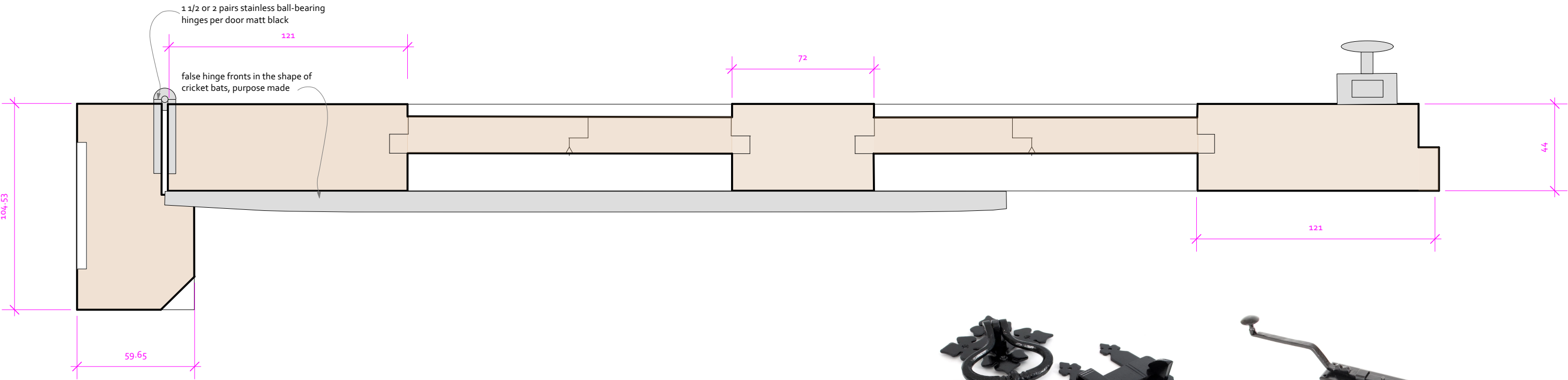
SECTION C-C showing frame section
