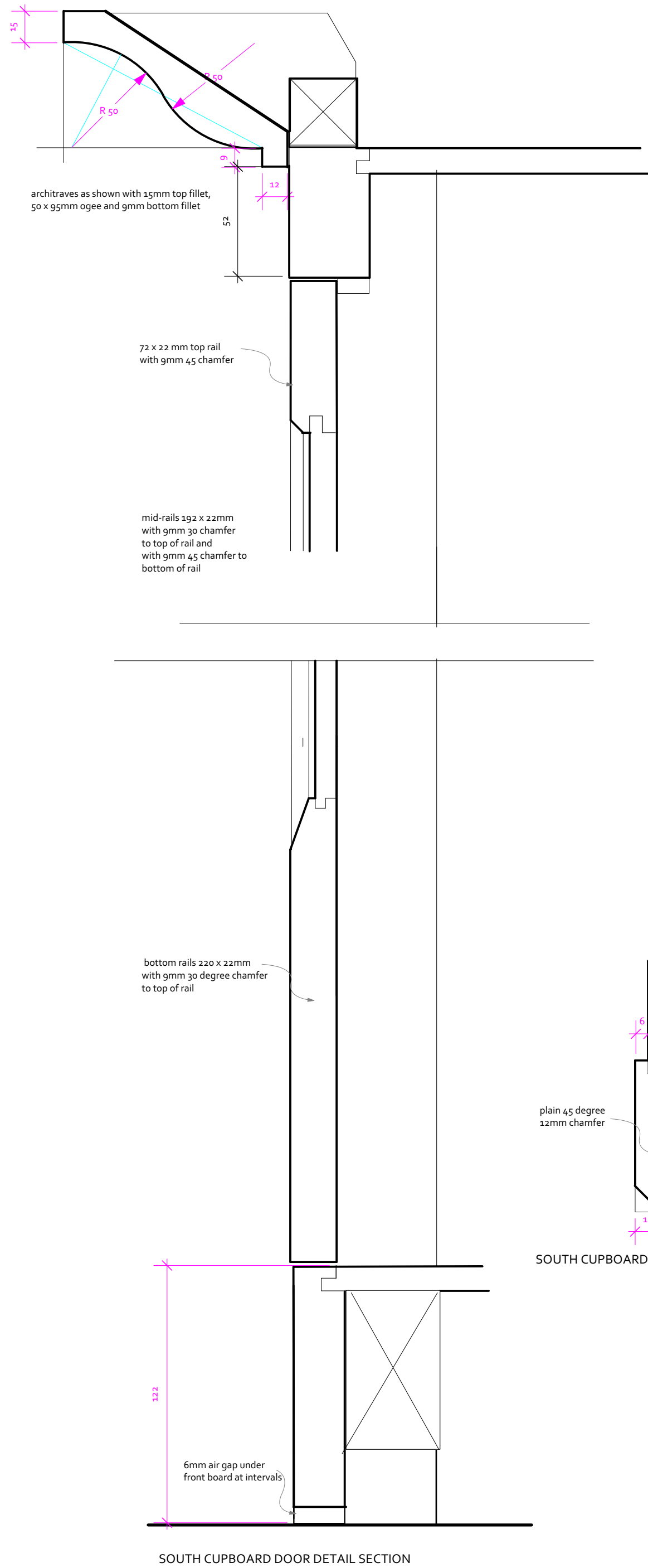
SOUTH CUPBOARD DOOR DETAIL SECTION
