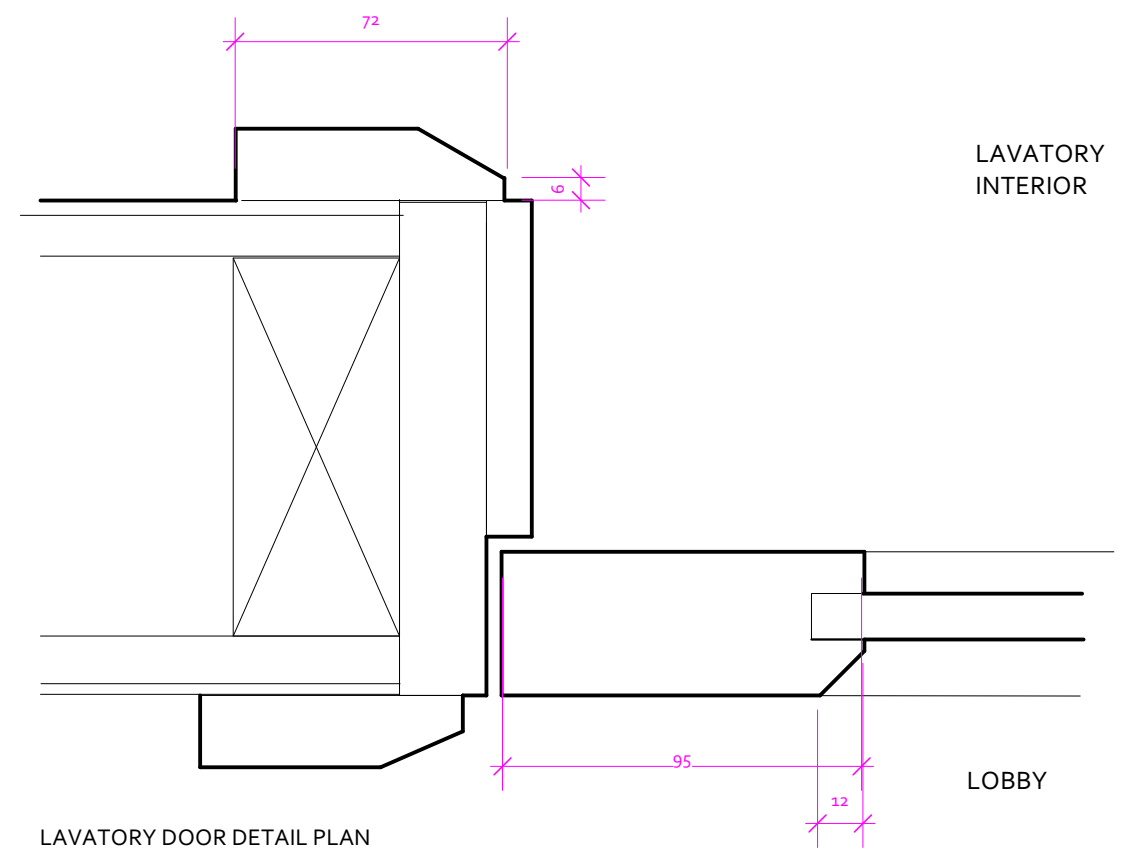
LAVATORY DOOR DETAIL PLAN
