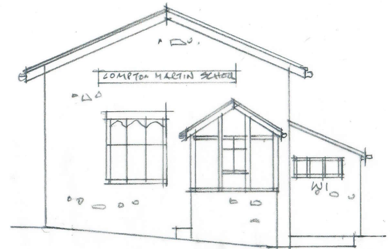
NORTH ELEVATION
