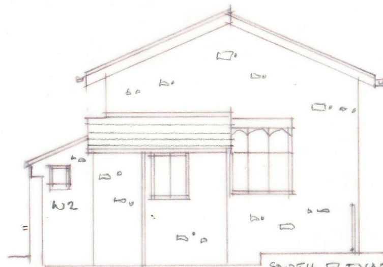
SOUTH ELEVATION
