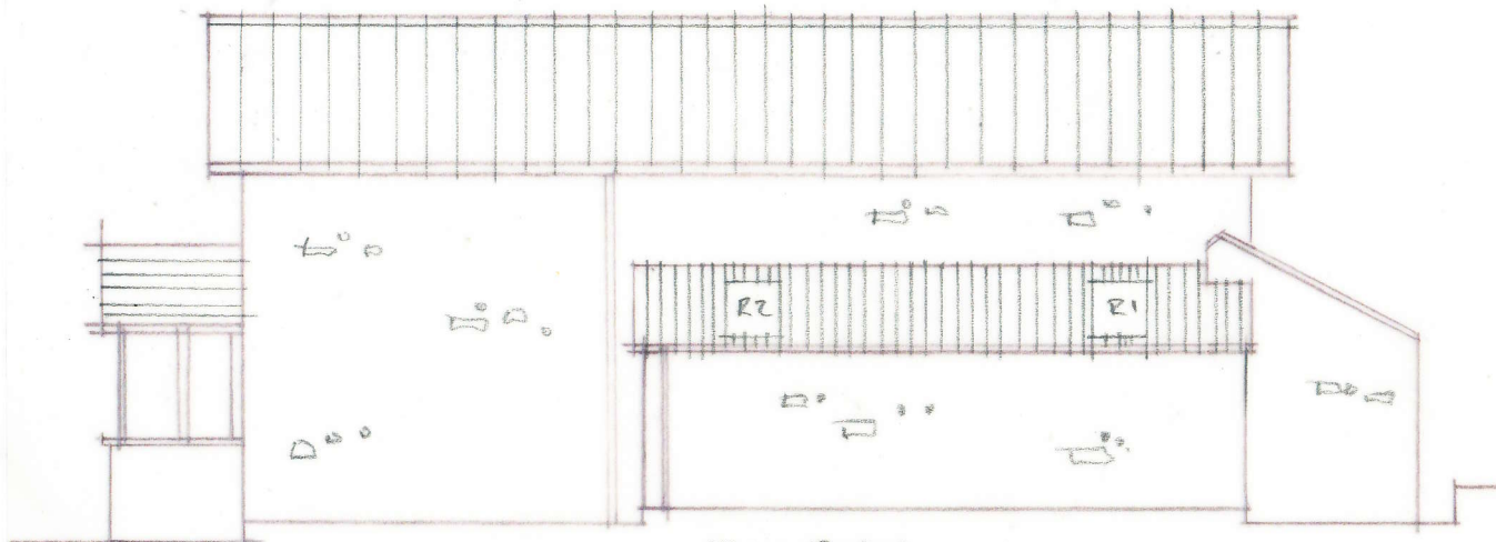
WEST ELEVATION
