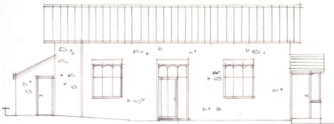
EAST ELEVATION
