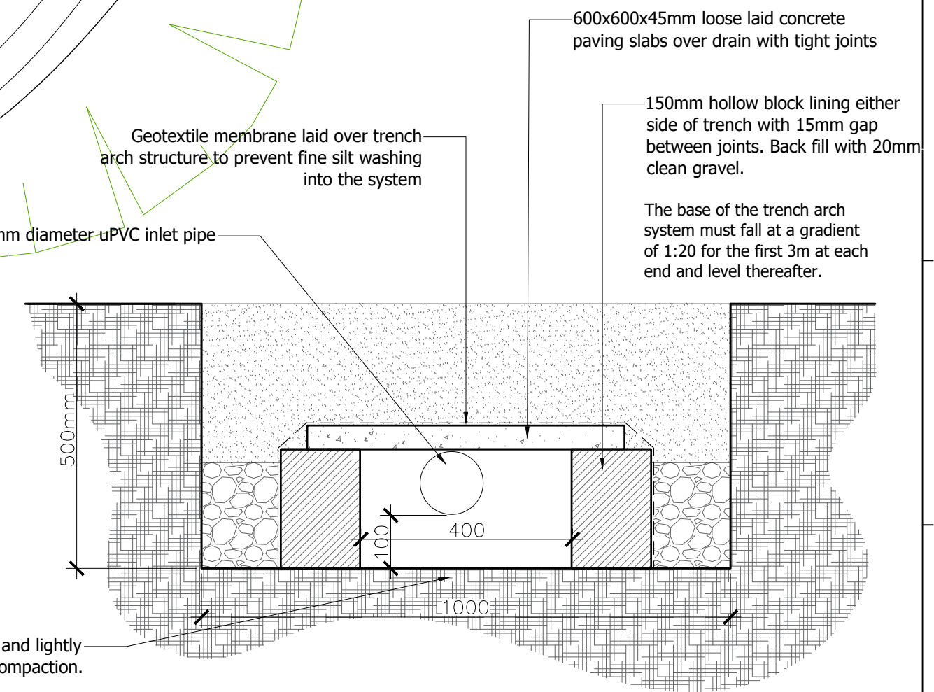
Cross Section Trench Arch System 1:10
