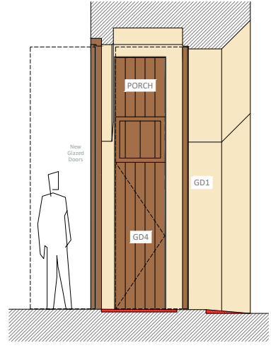
Central West Porch - Section A-A Sketch Option 3 - Scale 1:20
