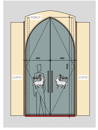
Central West Porch - Section B-B Sketch Option 3 - Scale 1:20
