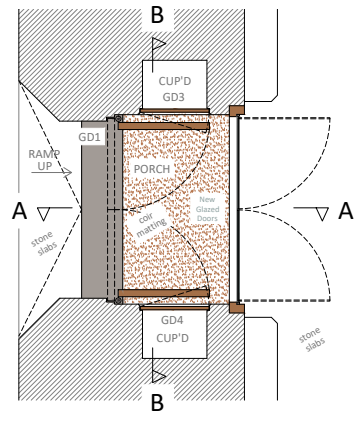
Central West Porch - Floor Plan Sketch Option 3 - Scale 1:20
