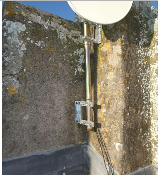
Bracket fixings to parapet and pinnacle base.
