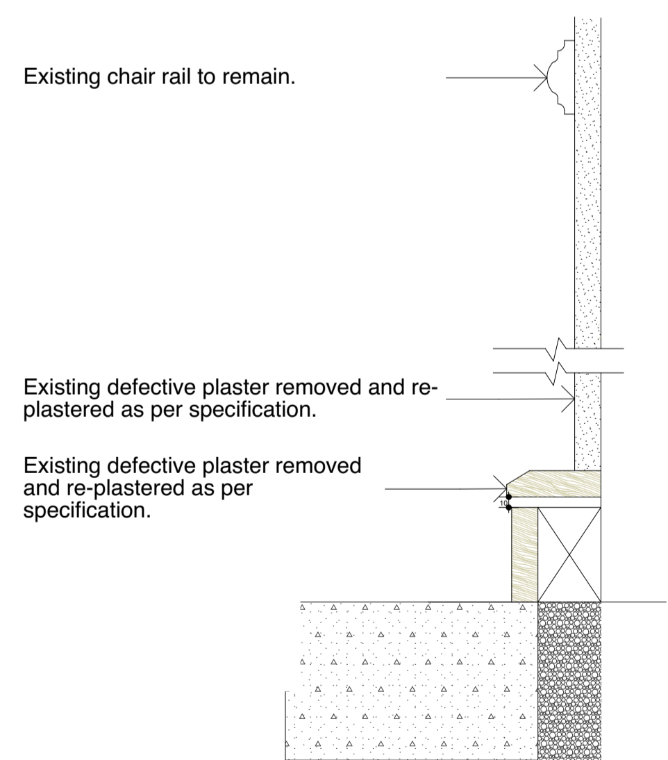
Detail A 1:5
