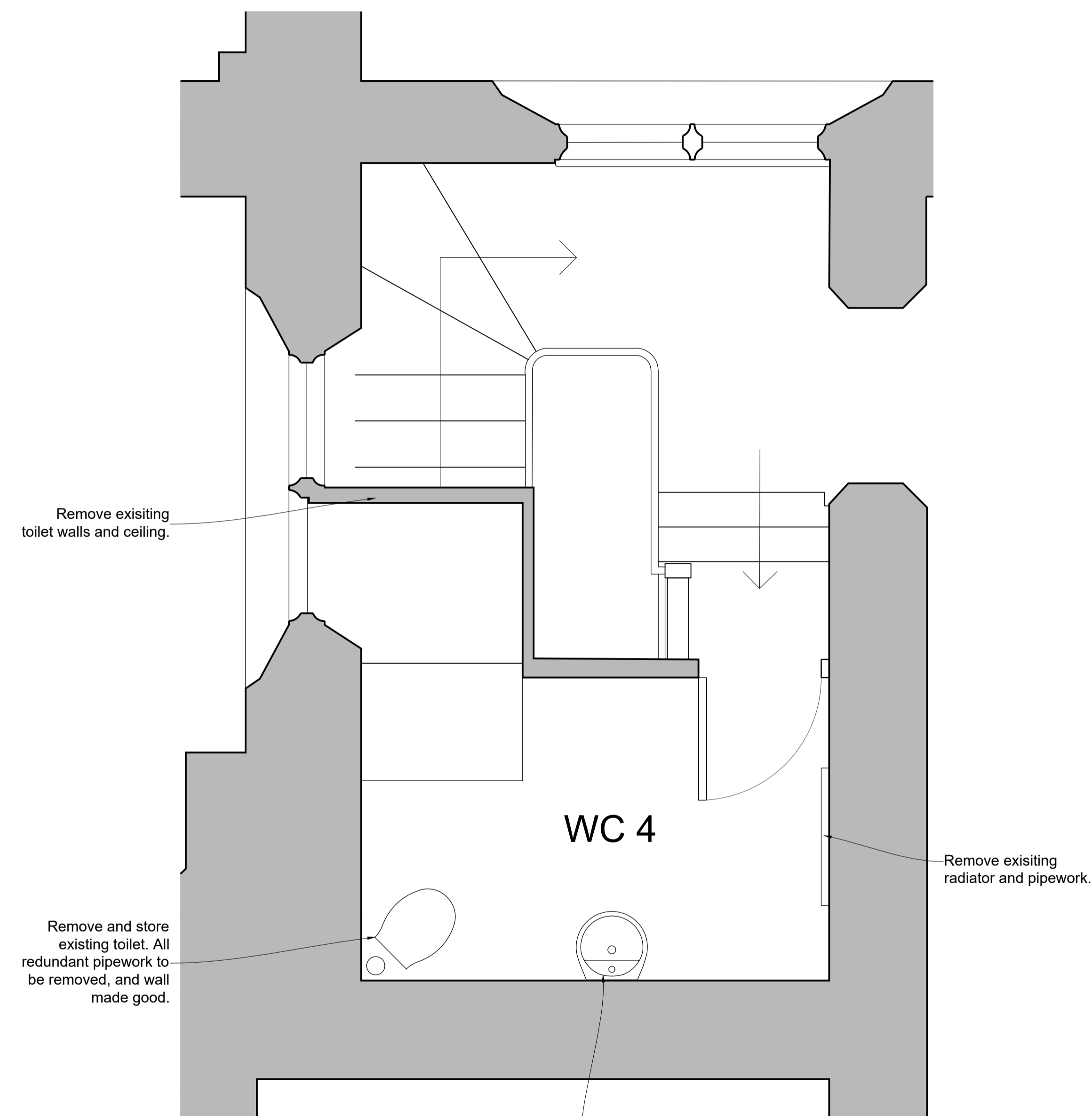
Mezzanine Floor Part Plan 1:20 As Existing
