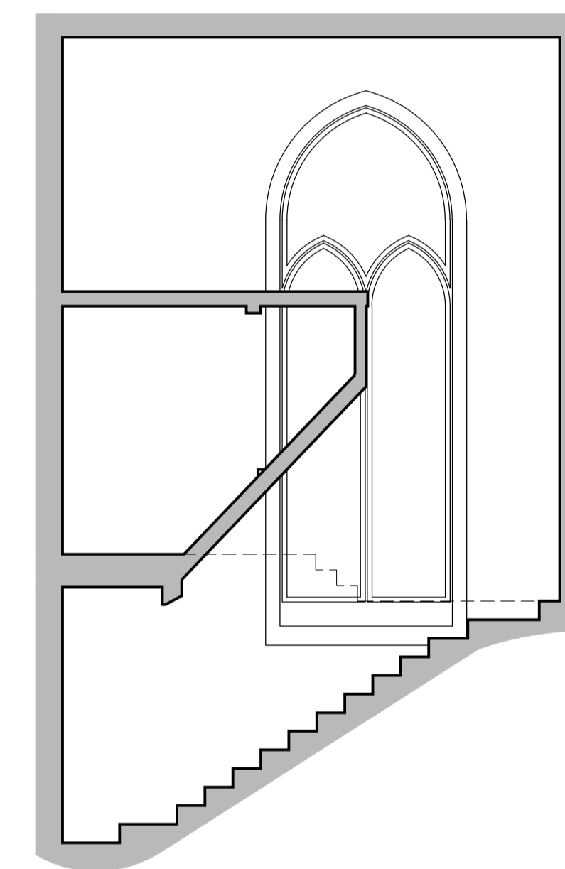
Mezzanine Floor Part Section A'A 1:50 As Existing
