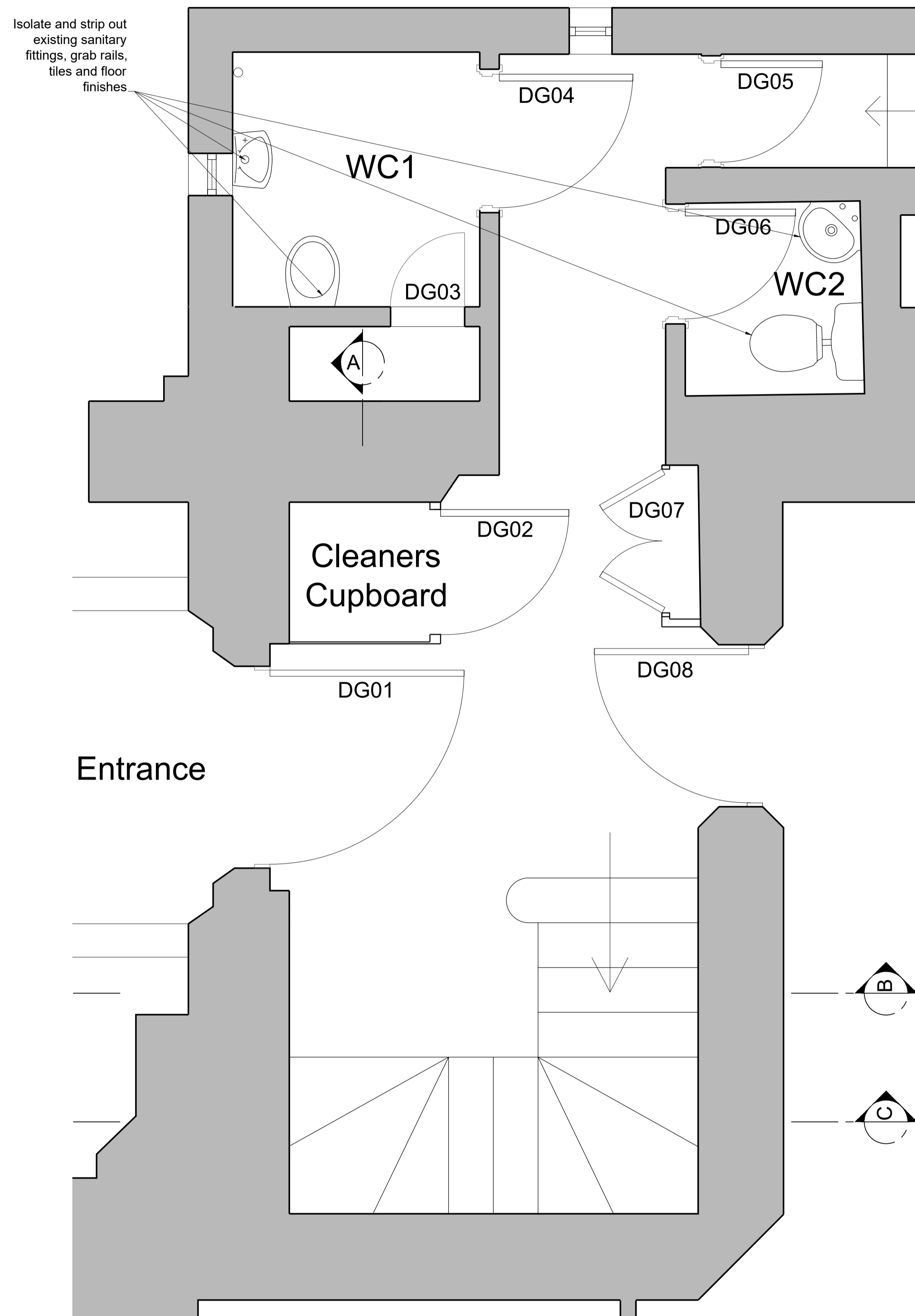
Ground Floor Part Plan 1:20 As Existing
