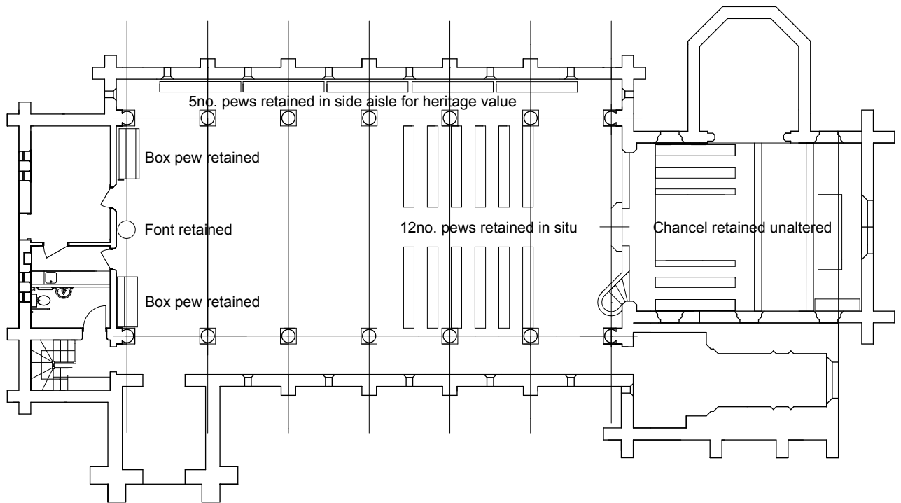
Ground Floor Plan-as proposed 1:200
