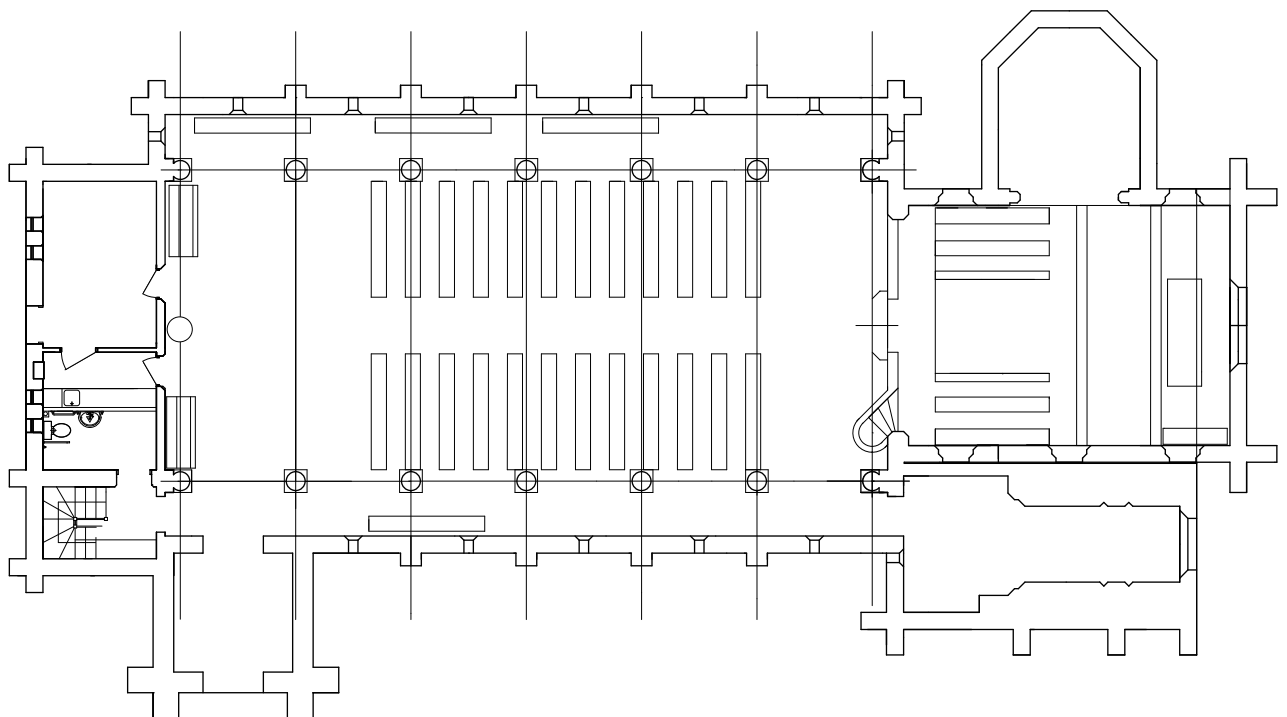
Ground Floor Plan-as existing 1:200
