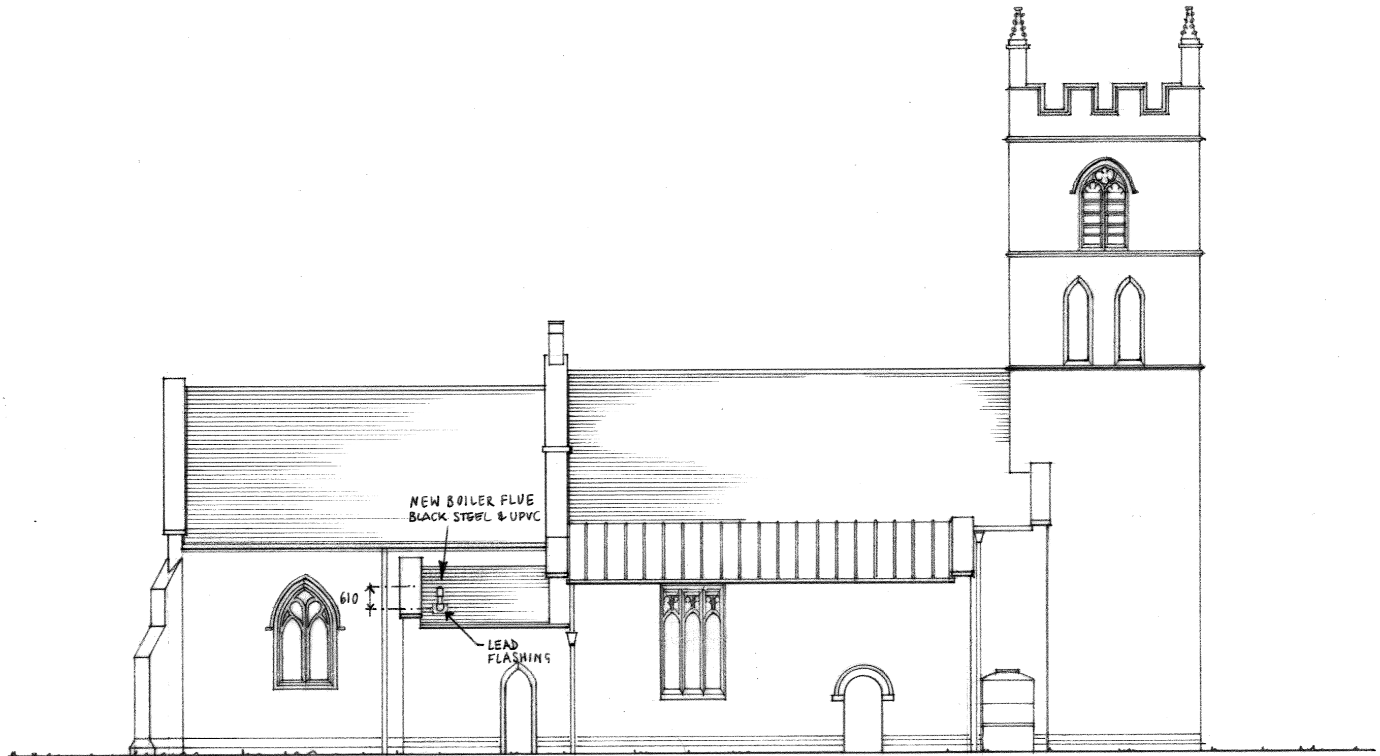
NORTH ELEVATION 1:100
